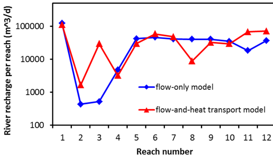
Figure 12: River recharge rates (m 3 /d) for each reach from (a) the flow model (blue line), and (b) the flow and heat transport model (red line).
