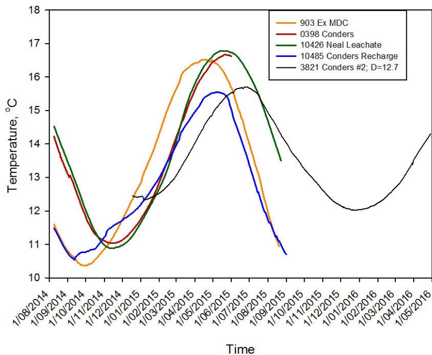
Figure 4: Mean daily temperature for sites with a temperature range between 3.5 and 6.5 °C.
