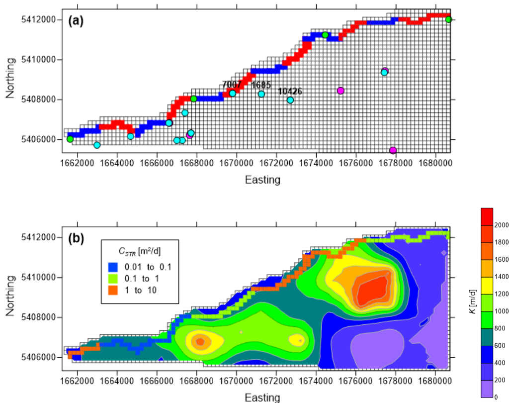
Figure 7: a) Model grid, river reaches (shown by alternating red-blue colours), and observation wells with groundwater-level data (purple circles), flow data (green circles), and temperature data (blue circles). (b) Spatially distributed hydraulic conductivity ( K ) and stream conductance ( C_{STR} ) values estimated through calibration.
