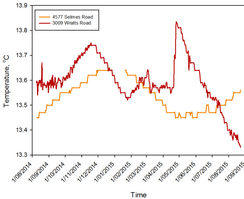
Figure 6: Mean daily temperature for sites with a temperature range less than 0.6 °C.
