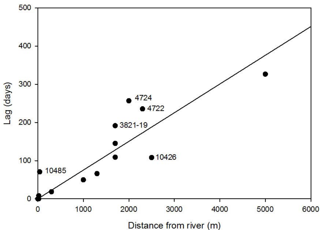
Figure 10: Variation of mean lag in temperature with distance from Wairau River.
