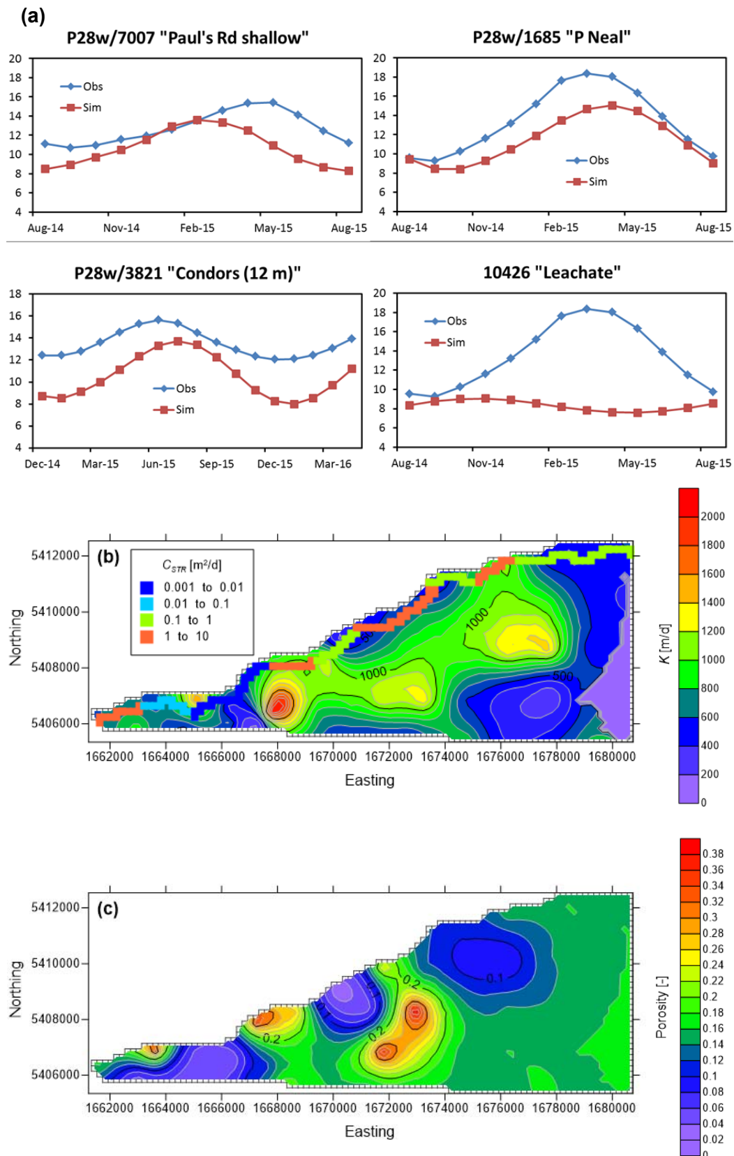
Figure 11: (a) Observed versus simulated temperature ( ^{\circ}\text{C} ) for wells P28w/7007, P28w/1685, P28w/3821, and 10426" (located 20, 1000, 1700, and 2500 m from river, respectively; Figure 1, Table 2), and spatially distributed (b) K for layer 11; i.e., the layer in which P28w/7007 and P28w/3821 targets are specified, and CSTR, and (c) \theta values for layer 11 estimated through calibration.
