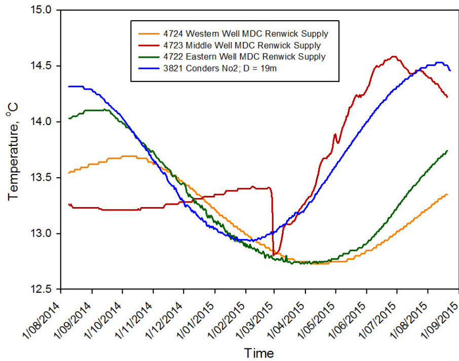
Figure 5: Mean daily temperature for sites with a temperature range between 0.9 and 1.8 °C.
