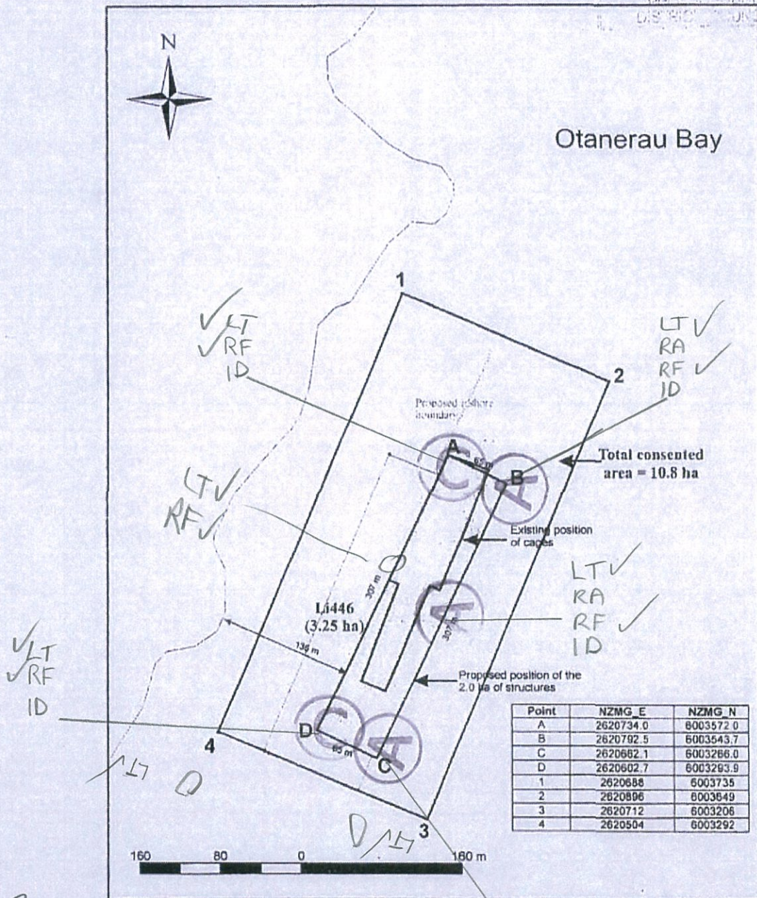
Figure 1: Proposed layout of the Otanerau Bay salmon farm (2.0), showing the present position of the farm.
