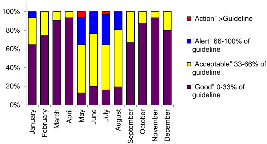
Figure 3.3: Comparison of daily PM 10 concentrations each month during 2020 to air quality indicator categories.
