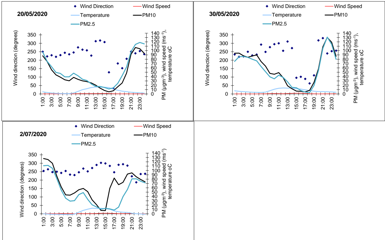
Figure 3.6: Hourly average PM 10 , PM 2.5 , wind direction and temperature on 20 th and 30 th May and 2 July 2020 when PM 10 concentrations exceeded 50 µg m -3 (24 hour average).
