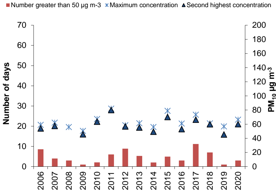
Figure 3.4: Number of days when 50 \mu\text{g m}^{-3} was exceeded, the maximum concentration and the second highest concentration from 2006 to 2020.
