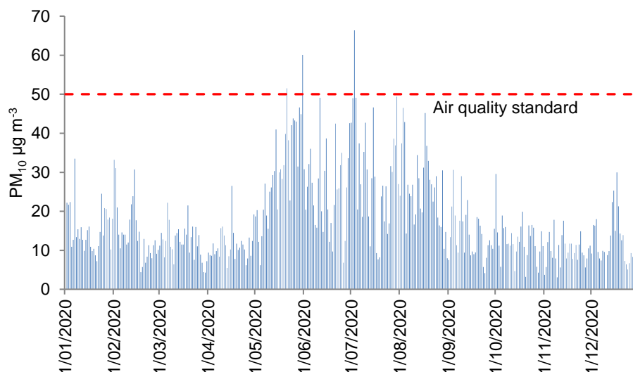
Figure 3.1: 24-hour average PM 10 concentrations measured at the Redwoodtown – Bowling Club site during 2020.
