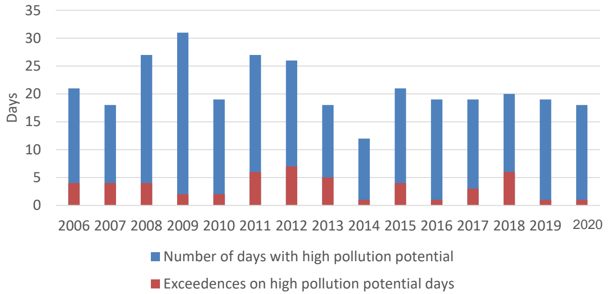
Figure 4.2: Prevalence of high pollution potential days and the number resulting in exceedences of 50 \mu\text{g}/\text{m}^3 (24-hour average) \text{PM}_{10} .
