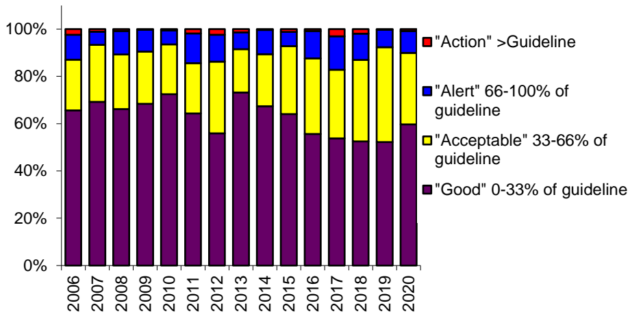
Figure 3.2: Comparison of PM 10 concentrations measured at Redwoodtown from 2006 to 2020 to air quality indicator categories.
