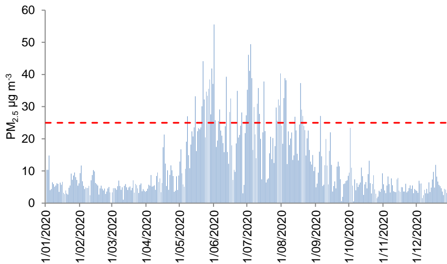
Figure 3.5: 24-hour average PM 2.5 concentrations measured at the Redwoodtown – Bowling Club site during 2020.
