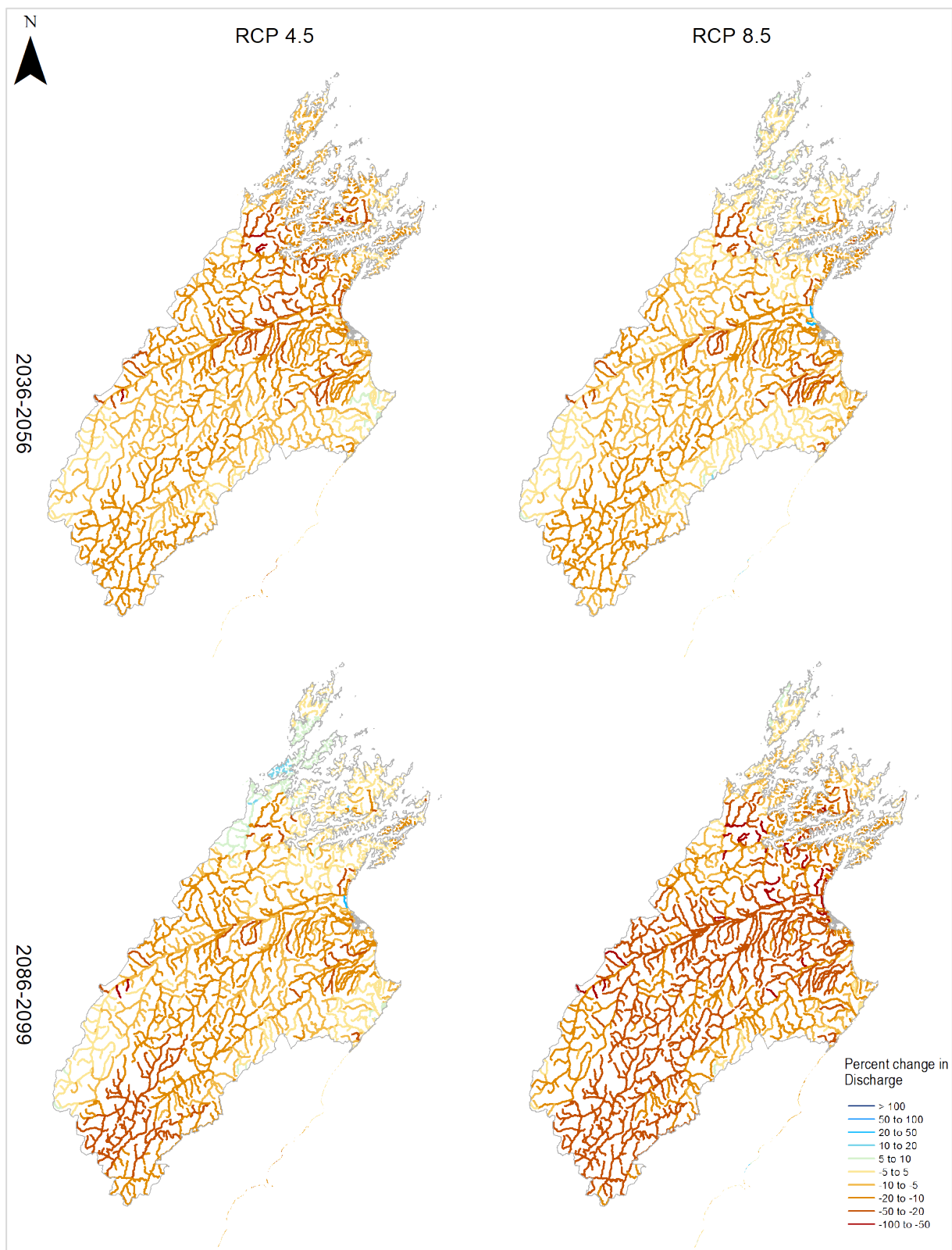
Figure 9-2: Percent changes in multi-model median of the mean annual low flow (MAF) across Marlborough for mid (top) and late-century (bottom). Climate change scenarios: RCP4.5 (left panels) and RCP8.5 (right panels). Time periods: mid-century (2036-2056) and end-century (2086-2099).
