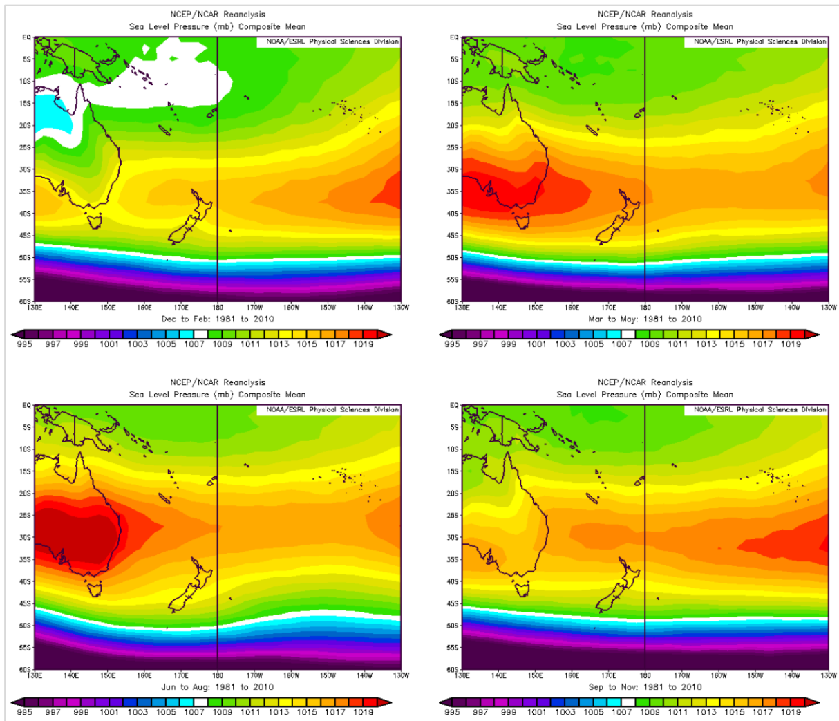
Figure 7-16: Average seasonal mean sea level pressure over the Southwest Pacific, 1981-2010. Top left: summer, top right: autumn, bottom left: winter, bottom right: spring. Sourced from:
