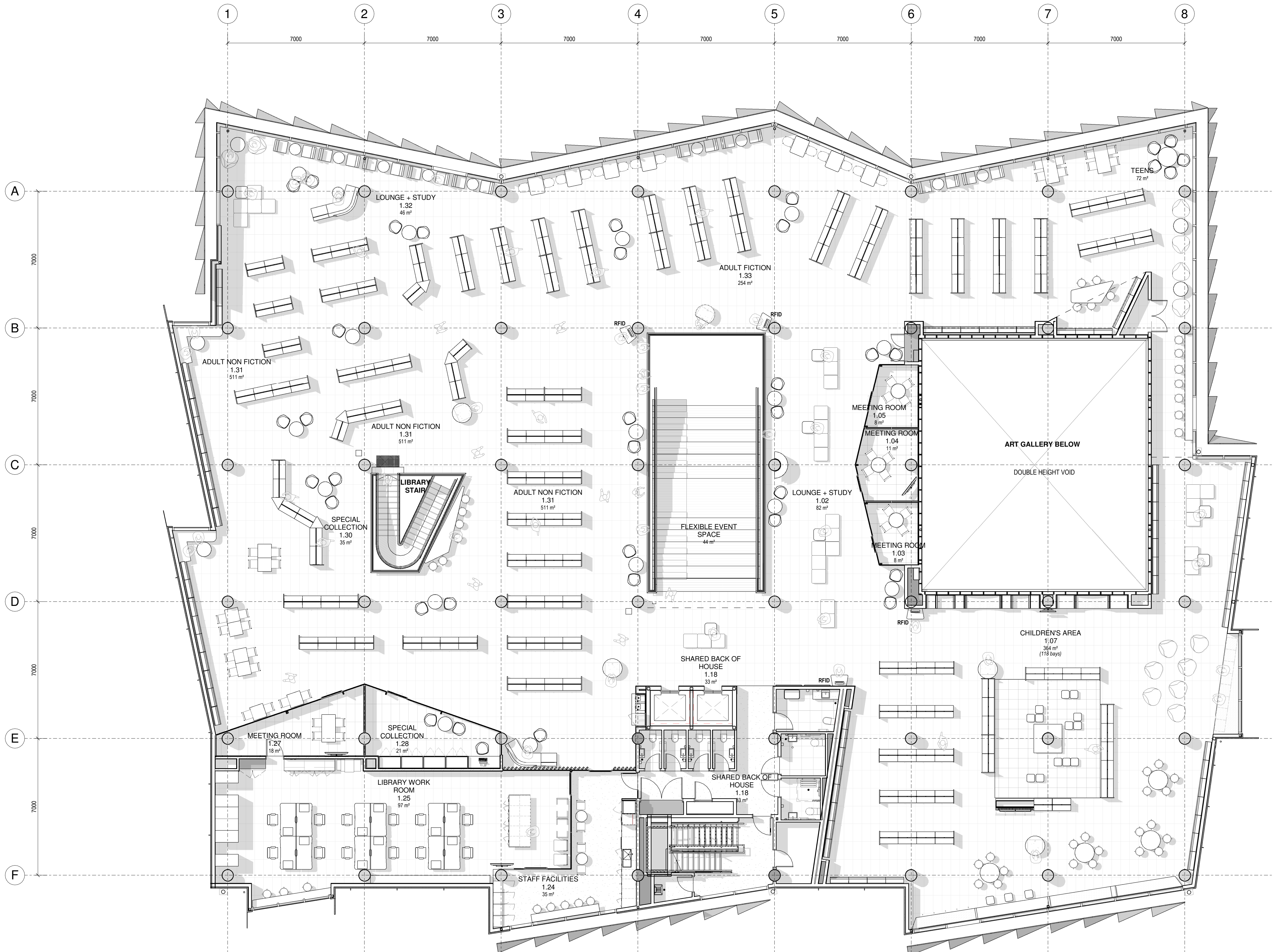
1 LEVEL 01 - FURNITURE PLAN A20.001 1:100
