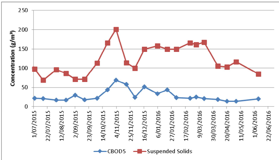
Figure 2-8: Wastewater monitoring results Pond 14 outlet – cBOD 5 and suspended solids
