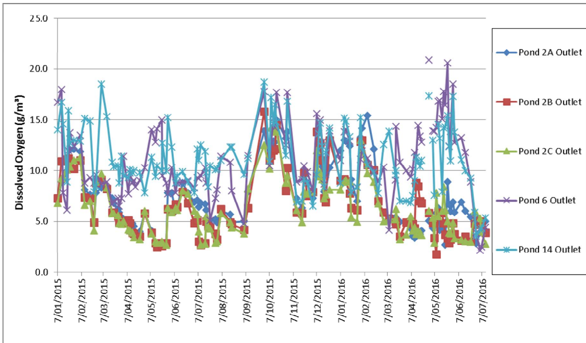
Figure 2-4: Dissolved oxygen monitoring results at the outlet of Ponds 2A, 2B, 2C, 6 and 14
