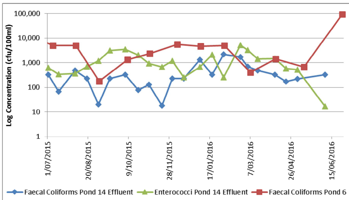
Figure 2-11: Wastewater monitoring results – Faecal coliforms at the outlet of Pond 6 and Faecal coliforms and Enterococci at Pond 14 on a Logarithmic Scale
