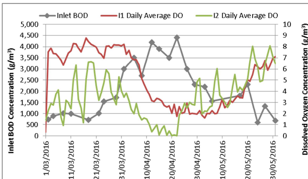
Figure 2-5: Dissolved oxygen daily averages in Ponds I1 and I2 compared to inlet BOD concentration
