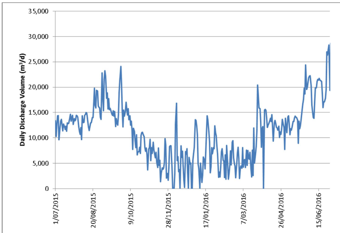
Figure 2-6: Daily discharge volume to Wairau Estuary
