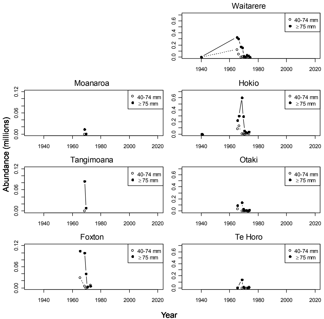
Figure 6: Estimated abundance of toheroa from surveys at seven beaches along the Manawatu/Kapiti coast west of Wellington from 1930 to present. Two shell length categories are plotted: 40–74 mm (open circles, dotted lines) and 75 mm or larger. Data from Tunbridge (1967, 1969) and Williamson (1969b, a, 1970, 1971, 1972, 1973).
