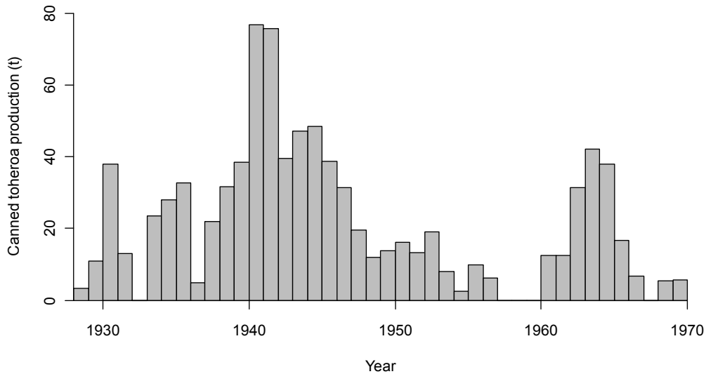
Figure 8: Total commercial production of toheroa (tonnes of canned toheroa product) from canneries at Northland beaches (Dargaville, Ninety Mile, and Muriwai) from 1928 to 1969. Data from Marine Department Annual records for 1928–40 and 1943–48 tabulated by Cassie (1955) and for 1941–42 and 1949–69 graphed by Redfearn (1974).
