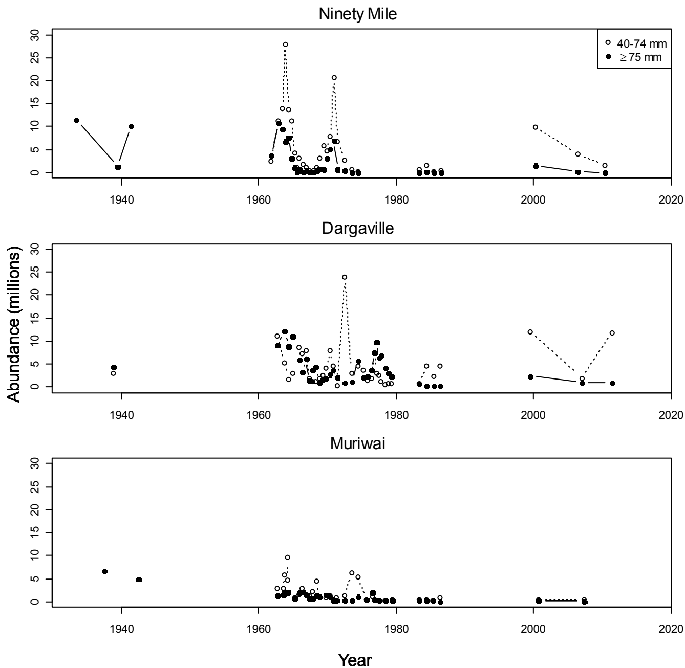
Figure 5: Estimated abundance of toheroa from surveys at Ninety Mile, Dargaville, and Muriwai beaches in Northland from 1930 to present. Two shell length categories are plotted: 40–74 mm (open circles, dotted lines) and 75 mm or larger. Data from Cassie (1955), Redfearn (1974), Greenway & Allen (1962), Greenway (1972, 1974), Akroyd et al. (2002, 2008), Morrison & Parkinson (2001, 2008), and Williams et al. (2013).
