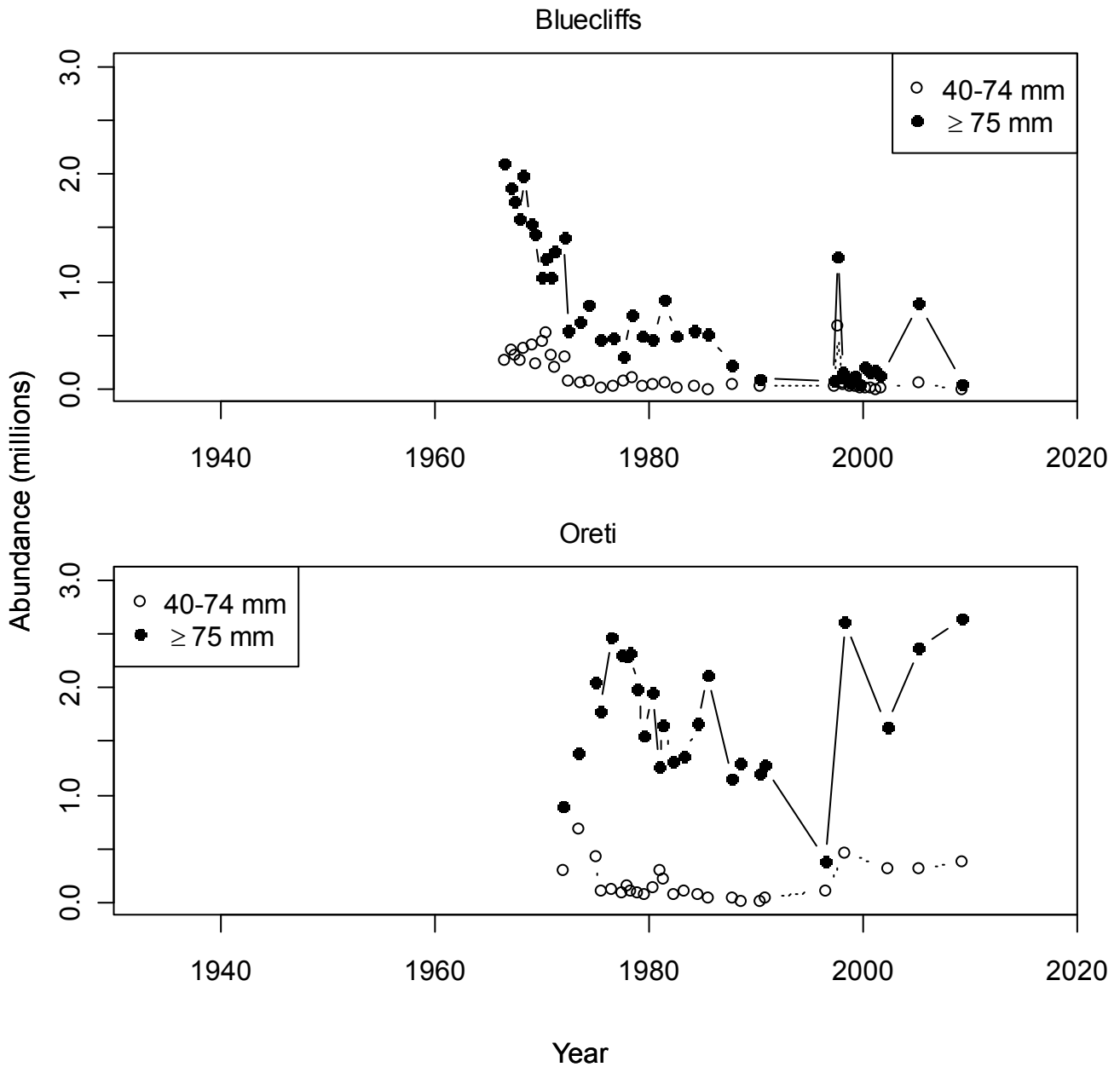
Figure 7: Estimated abundance of toheroa from surveys at Te Waewae and Oreti beaches in Southland from 1930 to present. Two shell length categories are plotted: 40–74 mm (open circles, dotted lines) and 75 mm or larger. Te Waewae data from Millar & Olsen (1995), Carbines (1997a), Carbines & Breen (1999a), Beentjes et al. (2003), Beentjes & Gilbert (2006a), and Beentjes (2010b). Oreti data from Street (1971, 1972), McKinnon & Olsen (1994), Carbines (1997b, 1998, 1999, 2000), Carbines & Breen (1999a), Beentjes & Carbines (2001), Beentjes & Gilbert (2006a), and Beentjes (2010a).
