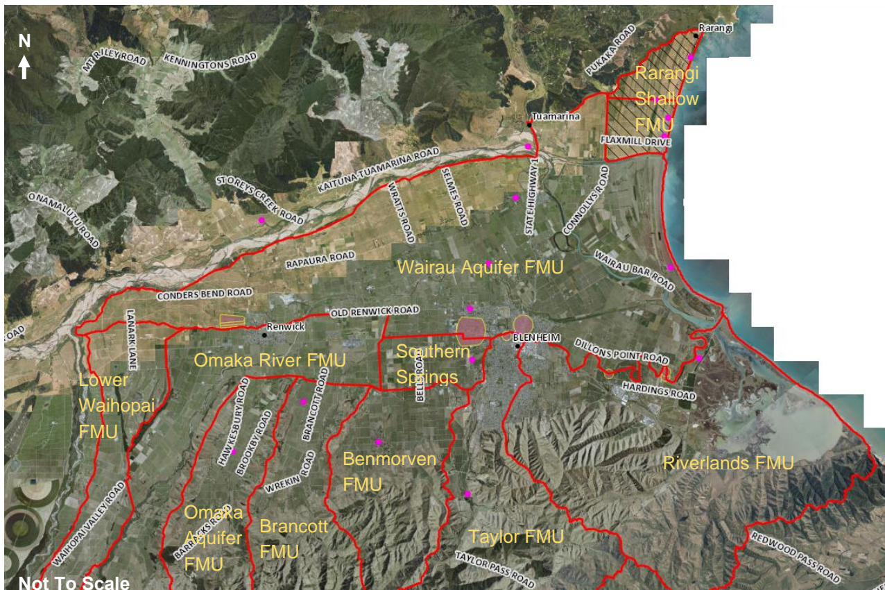
Figure 3: Freshwater Management Units (FMU) and groundwater protection zones (yellow/pink polygons) as per the pMEP.
