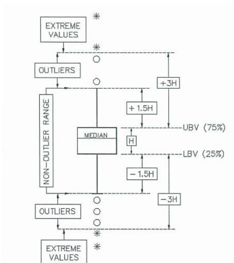
Figure 4 Typical properties of a box and whiskers plot (from Tonkin and Taylor 2006).
