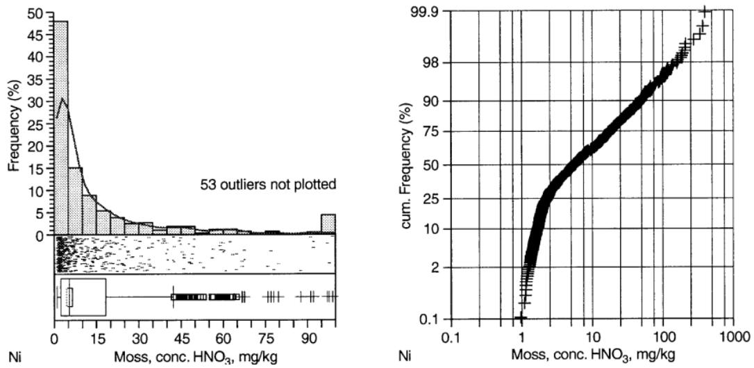
Figure 2 Combination of histogram, density trace, one-dimensional scattergram and boxplot and a CDF diagram to give a fast graphical impression of the data distribution (from Reimann & Filzmoser 2000).
