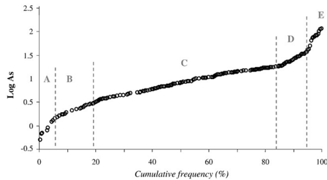
Figure 3 Cumulative frequency distribution curve of log-transformed data for arsenic, concentrations in Granada soils indicating the inflection points that separate the different classes (A, B, C, D and E) in the dataset. Dashed lines indicate the inflection points (from Diez et al. 2009).
