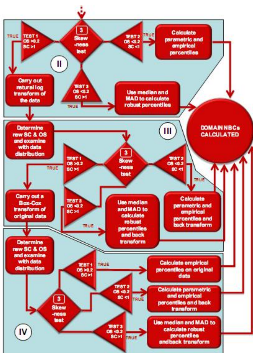
Figure 6 Statistical analysis outline used in Cave et al. (2012) to determine ‘normal’ background concentrations for defined domains.
