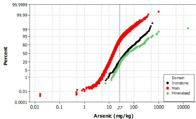
Figure 5 Probability plot of topsoil. Arsenic results categorised by potential domains. The k-means threshold of 27 mg/kg is shown by the vertical line. (Main = principal domain).
