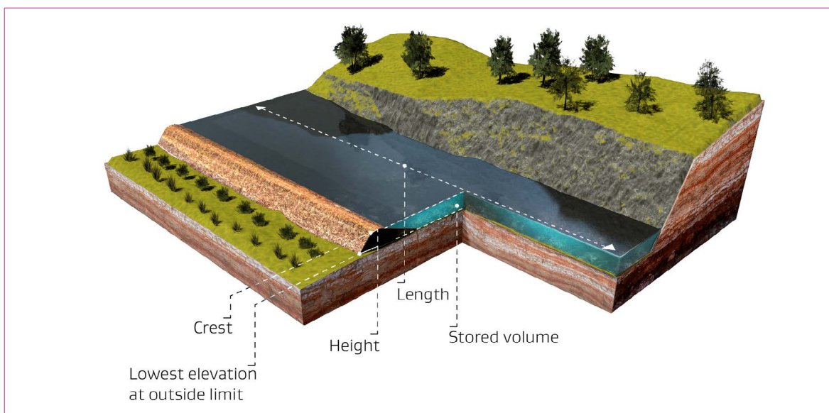
Figure 4: The typical cross-section of a canal dam with key features labelled.
