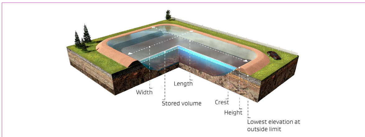
Figure 2: The typical cross-section of a rectangular dam with key features labelled.
