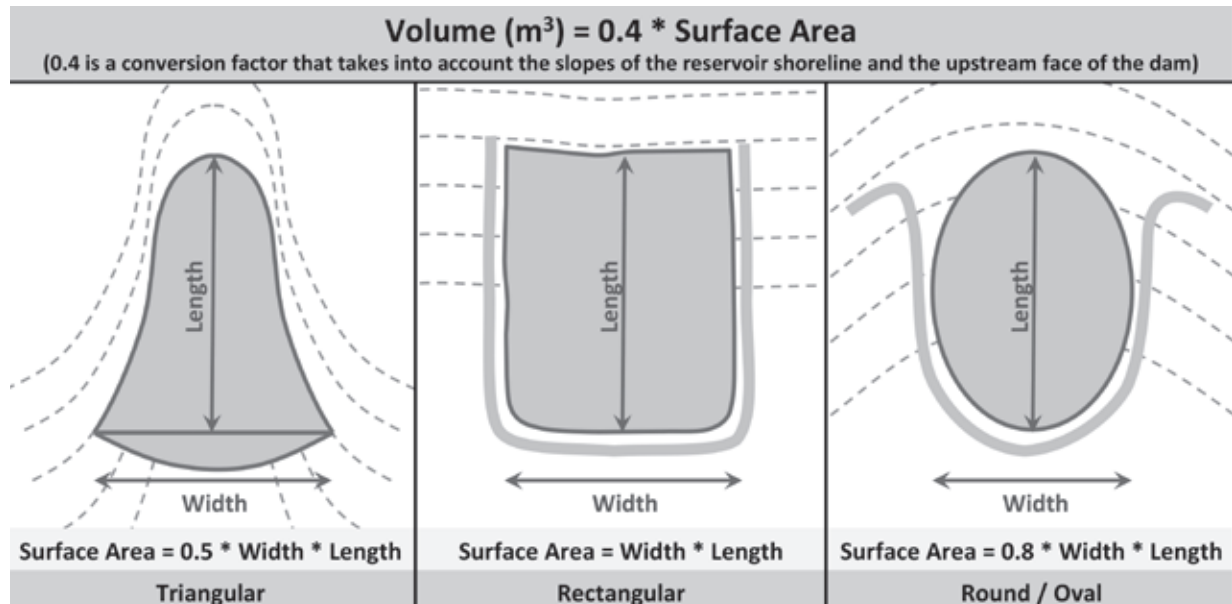
Figure 4.1: Simplified Calculation of Reservoir Volume
