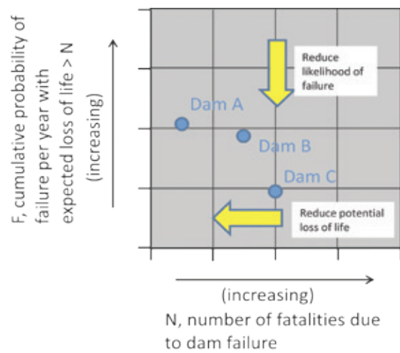
Figure 4.6: Risk Reduction Measures on Example F-N Plot
