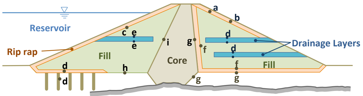
Figure 6.2: Critical and Non-Critical Filters (Redrafted from Fell et al 2005).
