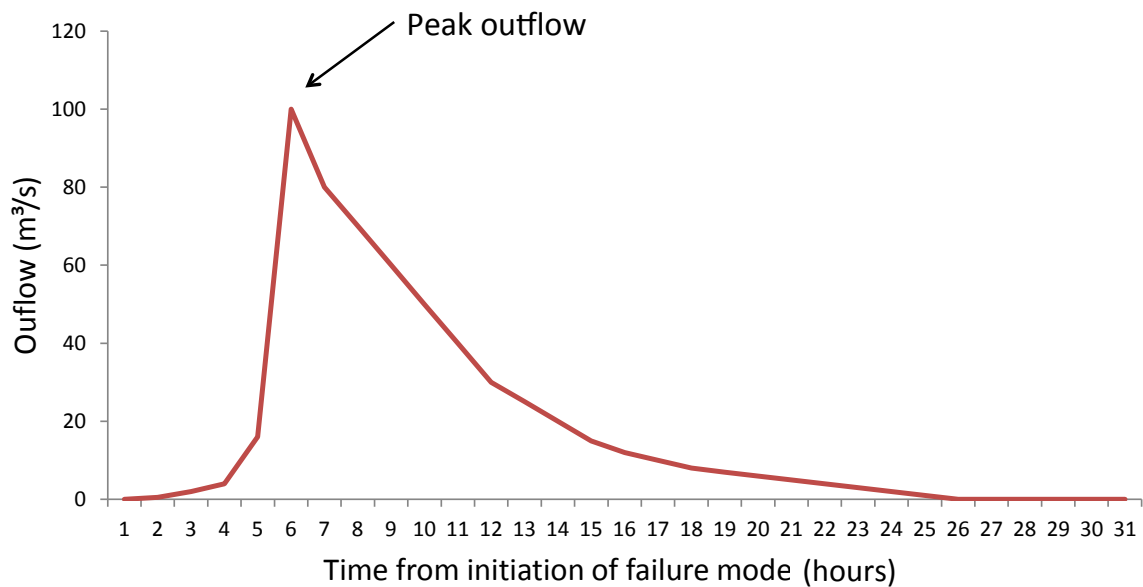
Figure 2.4: Example breach outflow hydrograph for a ‘sunny day’ failure of an earthfill or rockfill embankment dam
