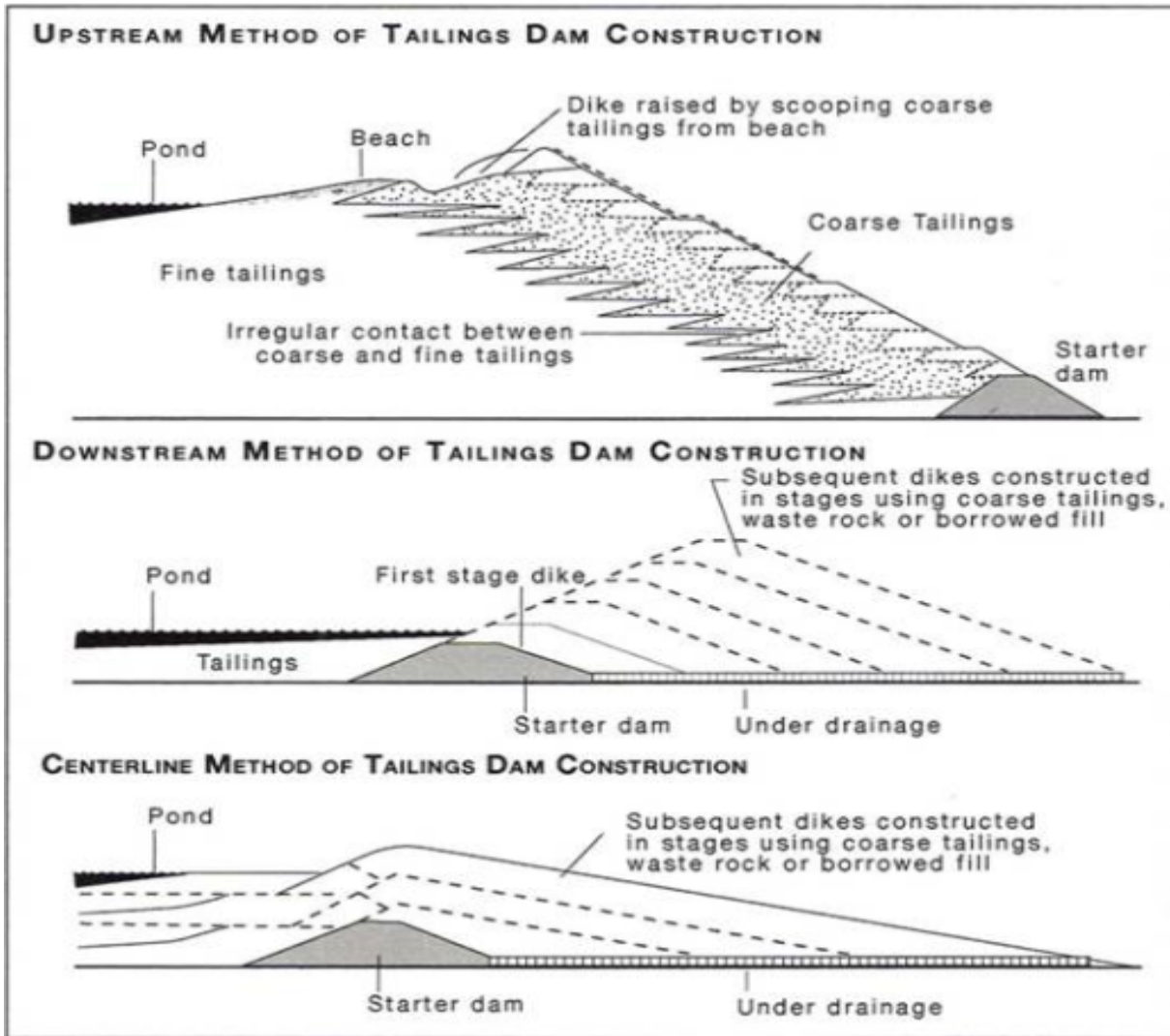
Figure 6.10: Tailings Dam Construction Methods
