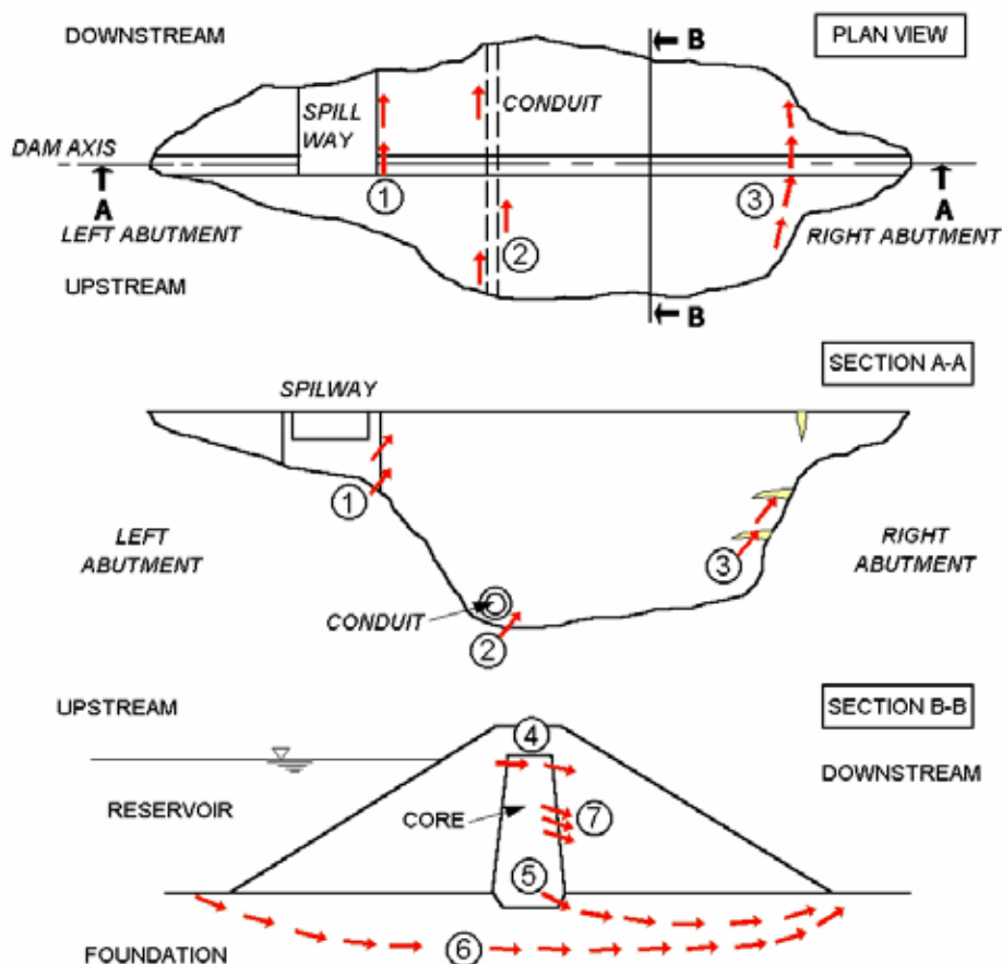
Figure 6.4: Possible Locations for the Initiation of Internal Erosion (from Fell and Fry 2007)
