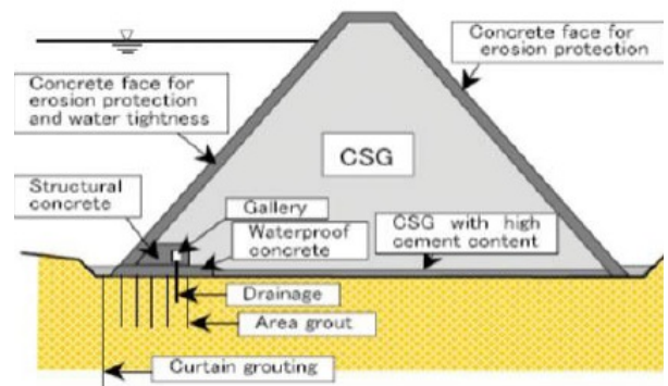
Figure 6.7: Hardfill Dam (CSG is Cement, Sand and Gravel)
