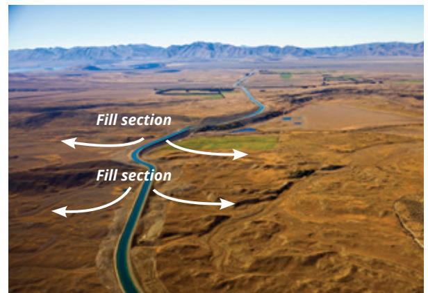
Figure 4.2: Example of Canal 'Fill' Sections with Different Features and Dam-Break Flow Paths. Copyright New Zealand Stock Library.
