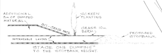
SECTION SHOWING DUMPING PROCEDURE. SCHEMATIC ONLY. REFER TO ORDINANCES.
